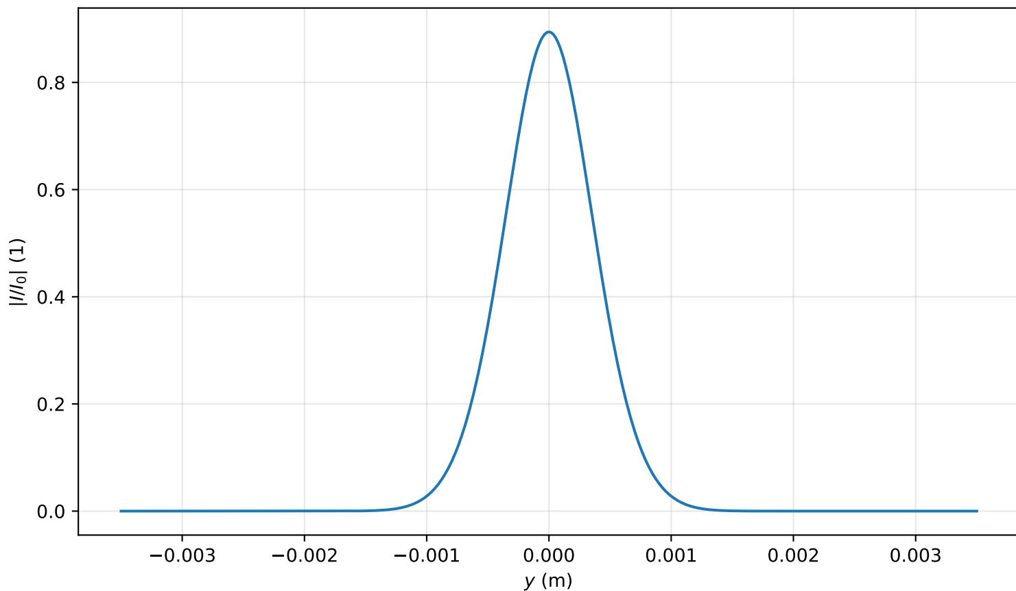
Intensity profile I(x=0, y, z=0.955)/I_0 , P_{in}=0.2P_{cr} , artificial time
